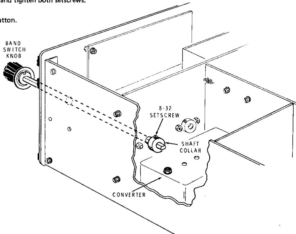
Detail 12-38A
