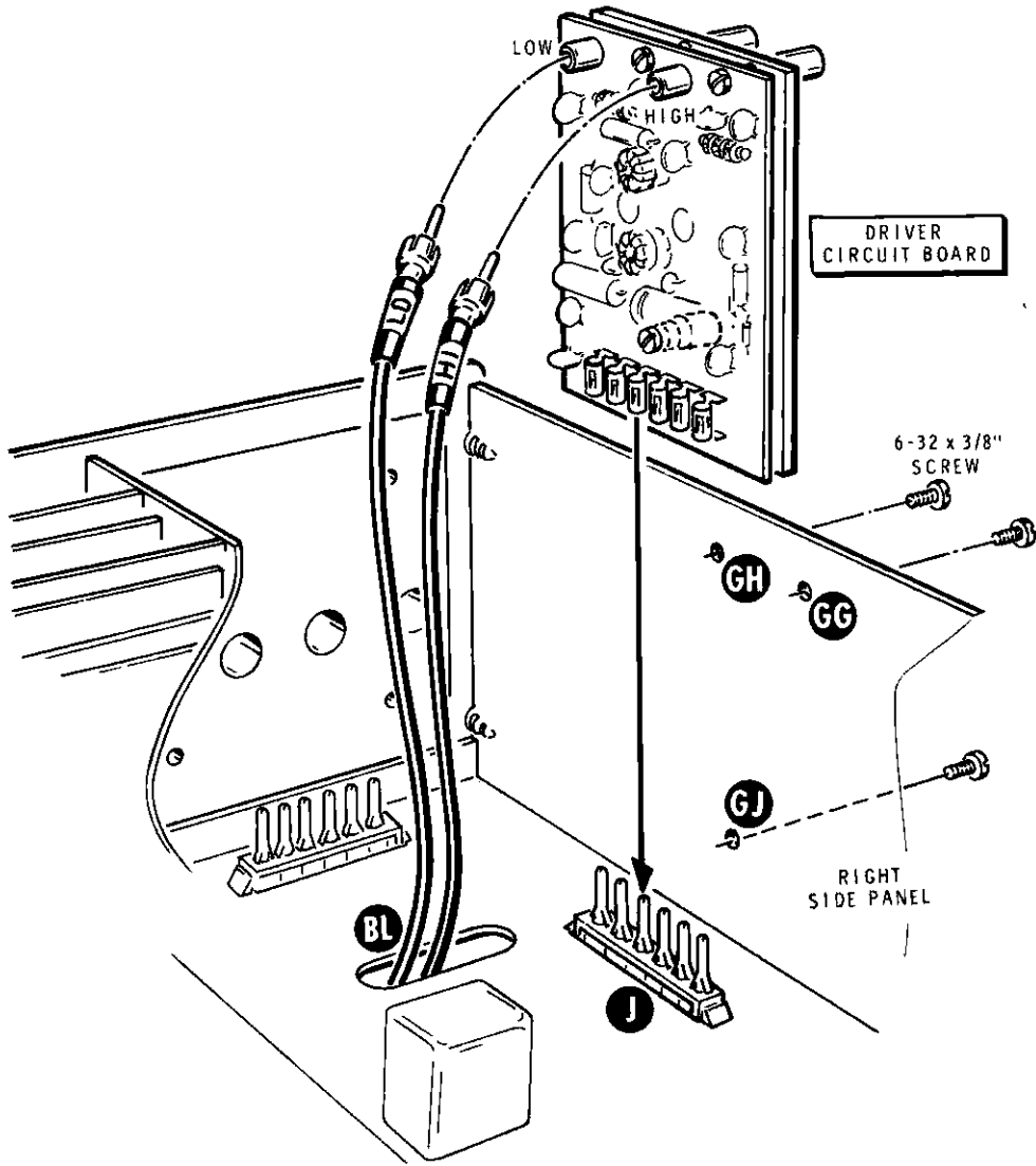
PICTORIAL 12-39
